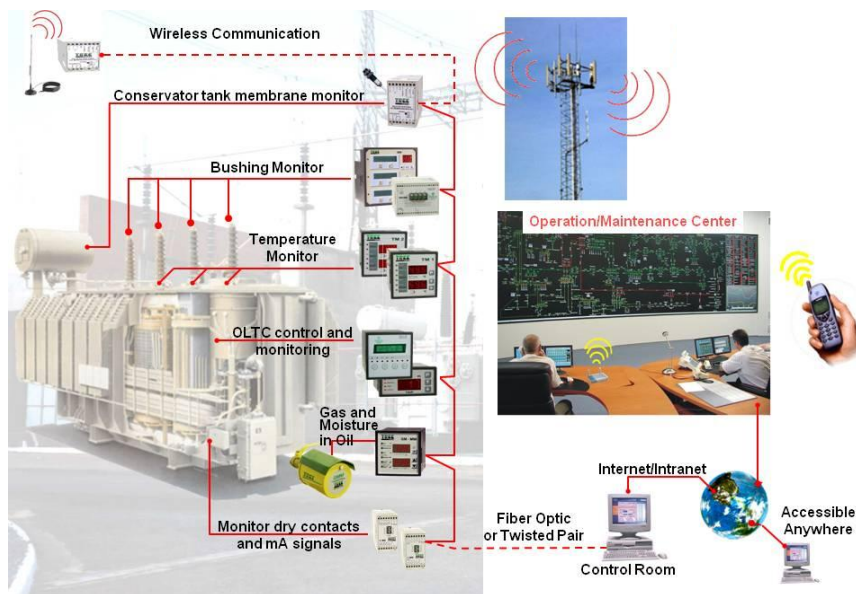
Figure 2- Architecture of the monitoring system
