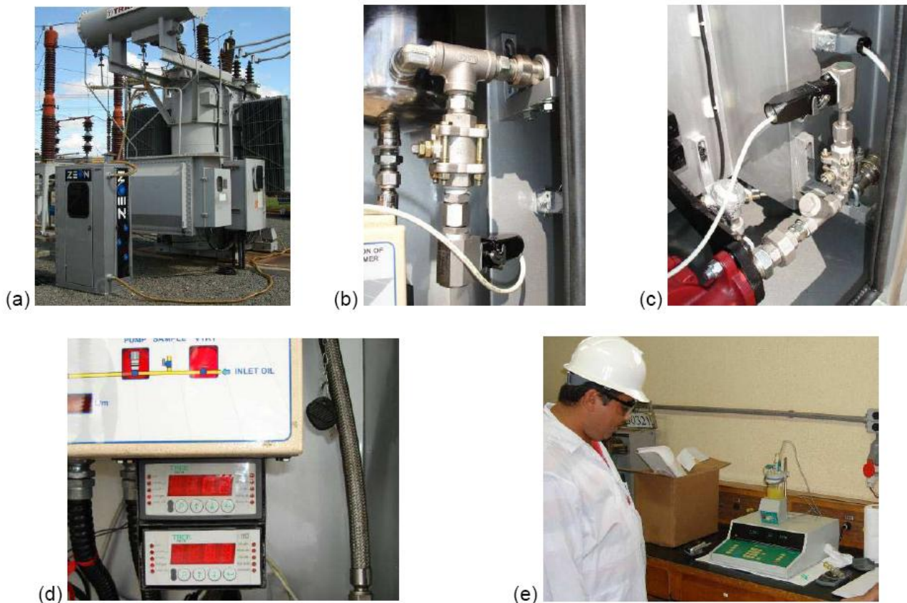
Figure 1 – Set up configuration; a) Zeon drying machine; b) MO Sensor at entrance to machine; c) MO Sensor at exit; d) interface modules; e) Metrohm Water Content Measurement Device.
