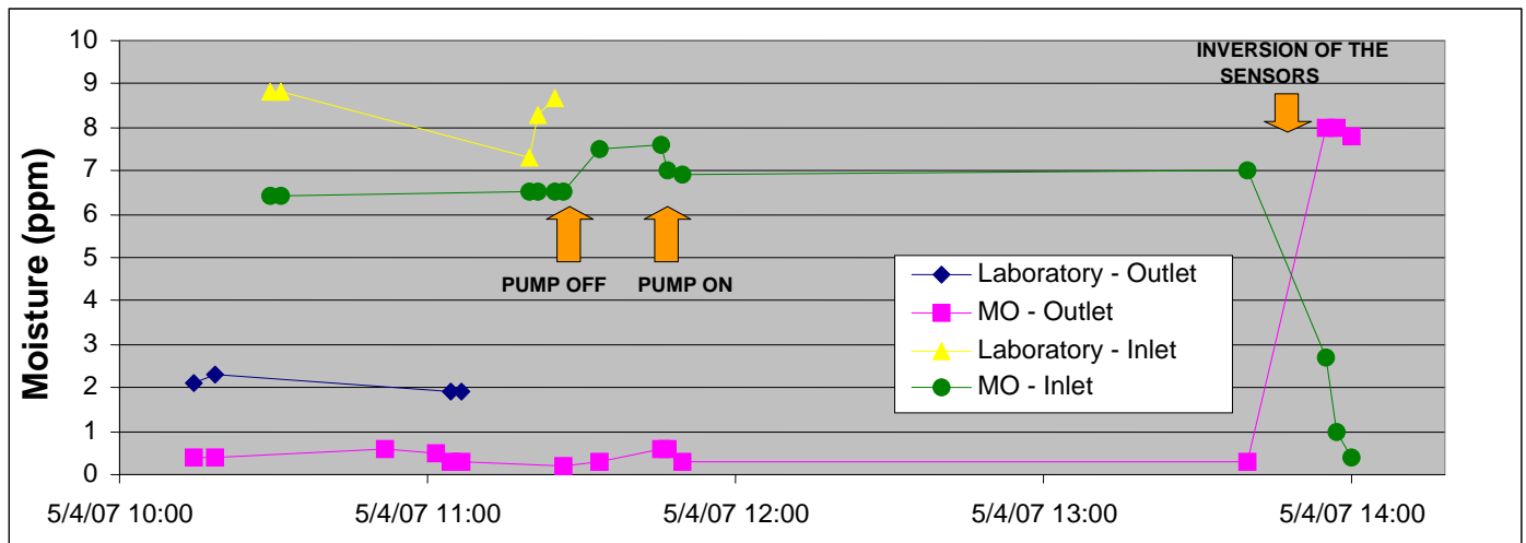
Figure 2 – Online and laboratory readings for water in oil content.
