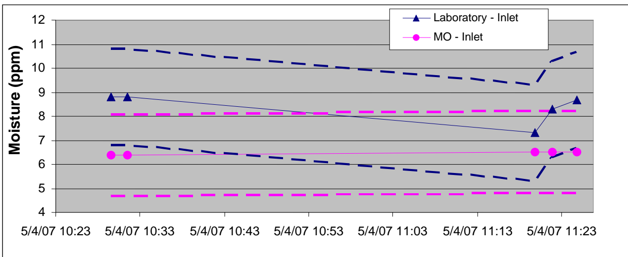
Figure 3 – Upper and lower tolerances of online and laboratory water content readings
