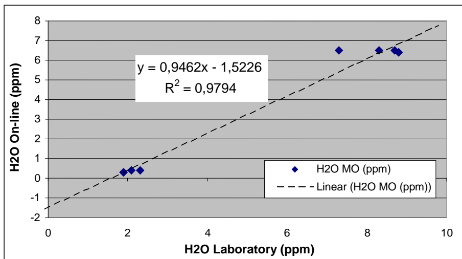
Figure 4 – Online water content readings as a function of laboratory readings.
