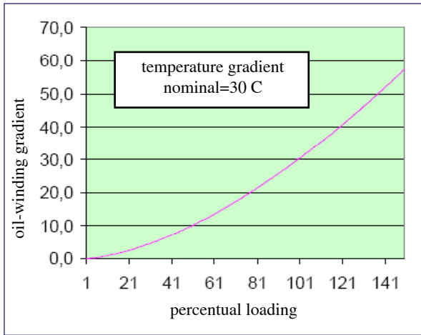
Figure 4 – Rise in winding-oil temperature as a function of the load
