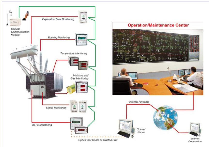
Figure 1 – Architecture of the monitoring system
