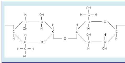
Figure 2 – Molecule of cellulose
