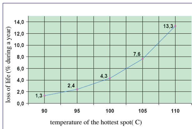
Figure 3 – Annual loss of life for insulation subjected to constant temperature
