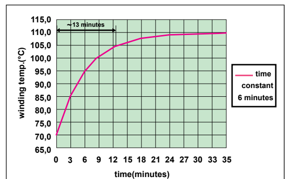
Figure 5 – Evolution of winding temperature in time
